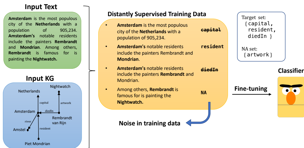
Figure 1: Overview of Distantly Supervised Relation Extraction. The first and third generated training examples are incorrect, the second and fourth ones are correct.
